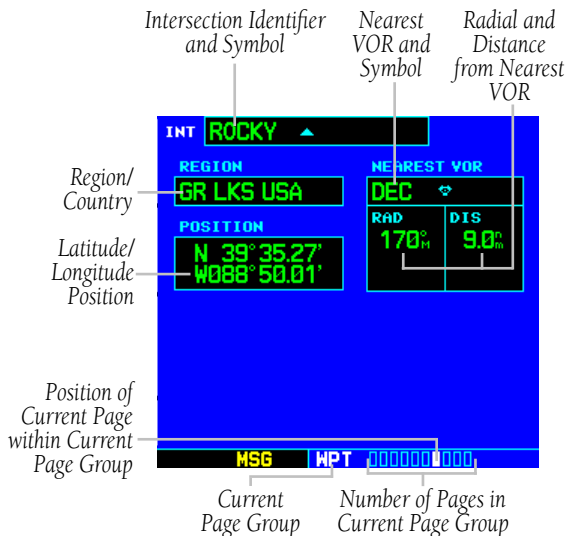
Figure 7-32 Intersection Page
